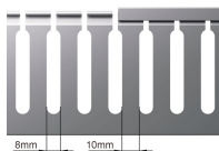
Wide Slot (L) 宽齿(L)
